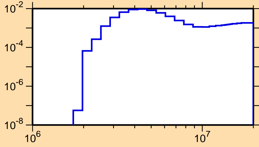
\sigma vs. E for ^{104}\text{Sn}(n,n\text{cont.})
