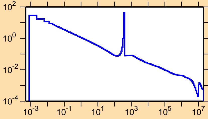
\sigma vs. E for ^{104}\text{Sn}(n,\gamma)
