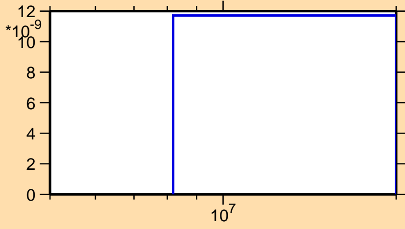
\sigma vs. E for ^{104}\text{Sn}(\text{mt117})
