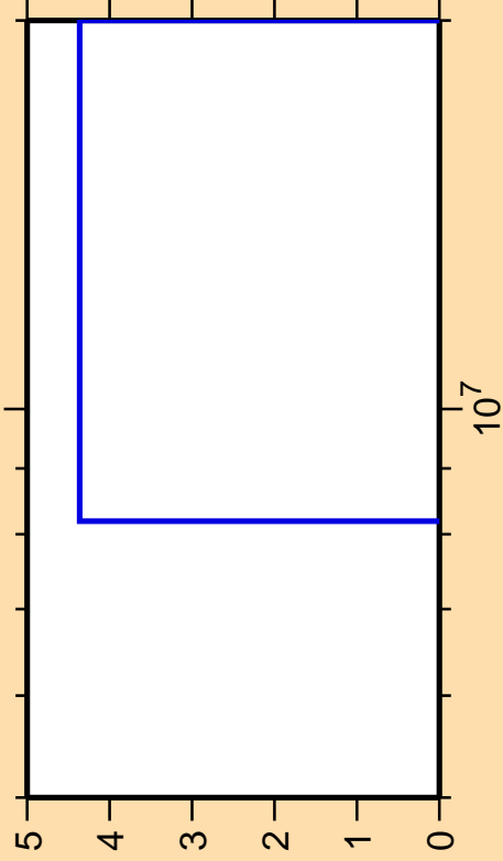
\Delta\sigma/\sigma vs. E for ^{104}\text{Sn}(n,2n\alpha)
