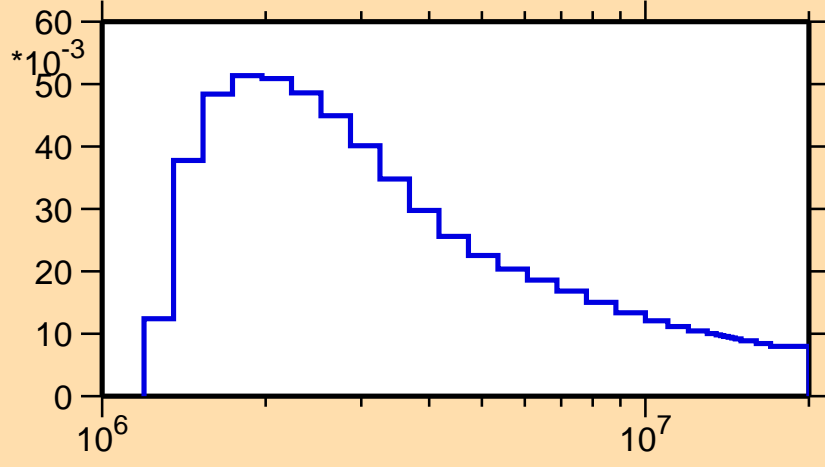
\sigma vs. E for ^{105}\text{Sn}(n,n_2)
