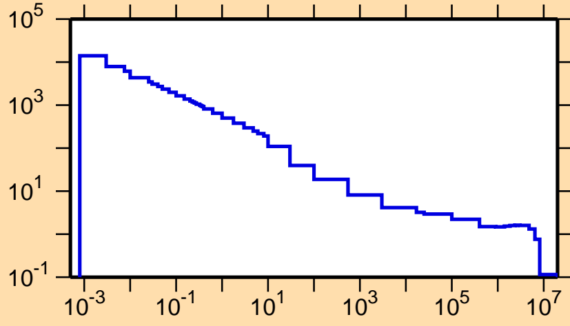
\sigma vs. E for ^{105}\text{Sn}(n,p)
