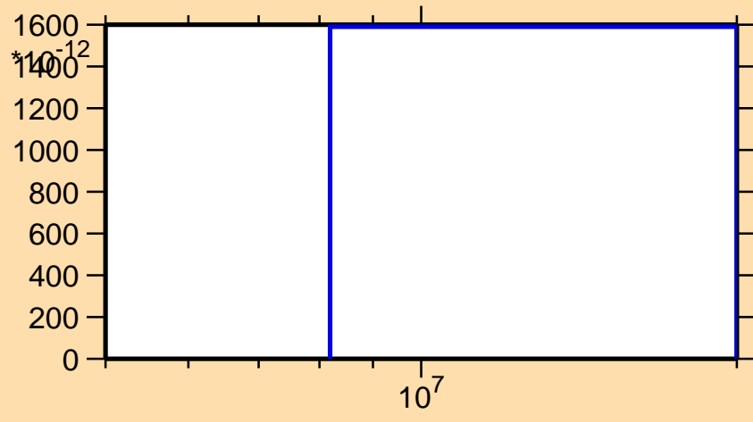
\sigma vs. E for ^{105}\text{Sn}(\text{mt } 34)
