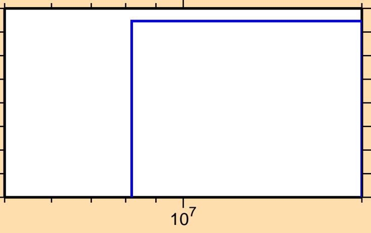
\sigma vs. E for ^{105}\text{Sn}(n,2n\alpha)
