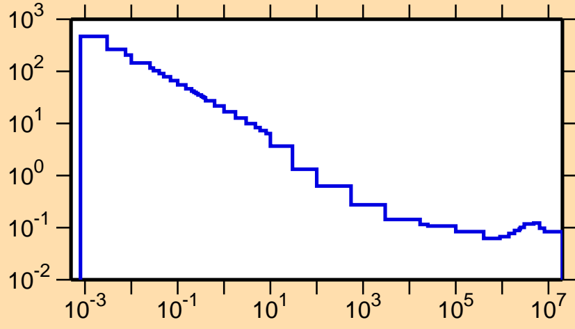
\sigma vs. E for ^{105}\text{Sn}(n,\alpha)
