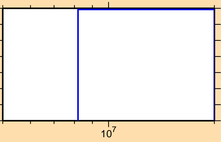
\sigma vs. E for ^{106}\text{Sn}(n,\text{pd})
