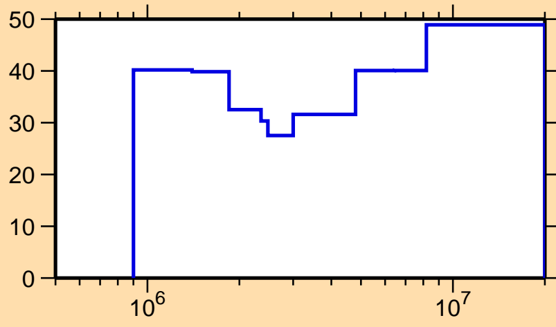
\Delta\sigma/\sigma vs. E for ^{106}\text{Sn}(n,n_1)
