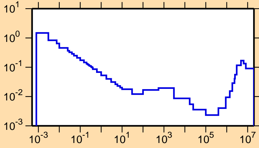
\sigma vs. E for ^{106}\text{Sn}(n,\alpha)
