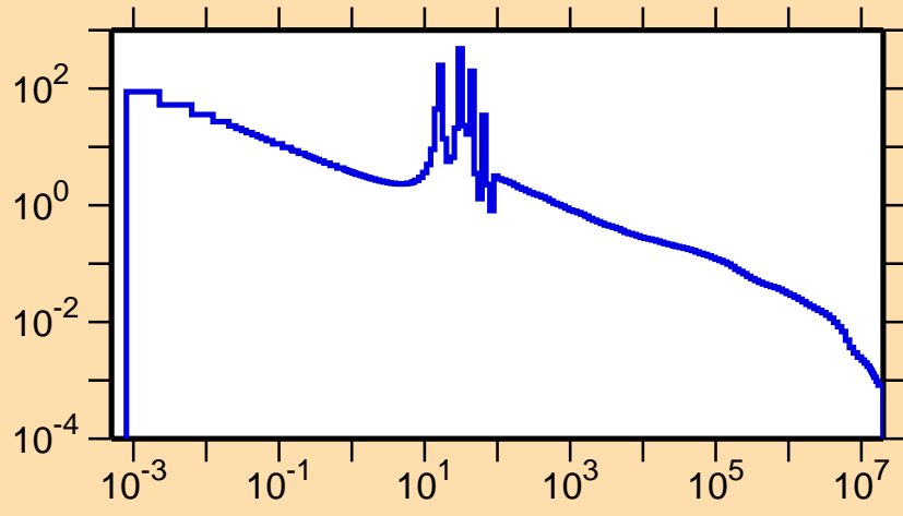
\sigma vs. E for ^{107}\text{Sn}(n,\gamma)
