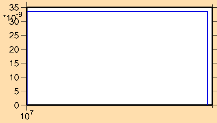
\sigma vs. E for ^{107}\text{Sn} (mt 45)
