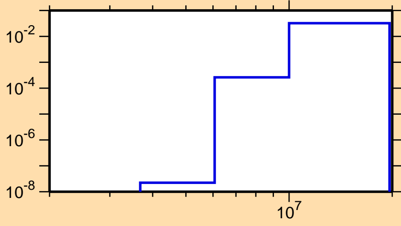
\sigma vs. E for ^{107}\text{Sn}(n,n\alpha)
