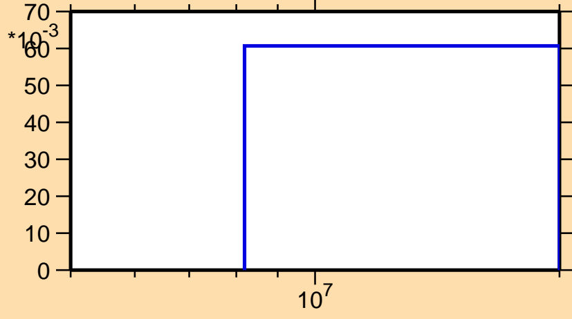
\sigma vs. E for ^{107}\text{Sn}(n,2n)
