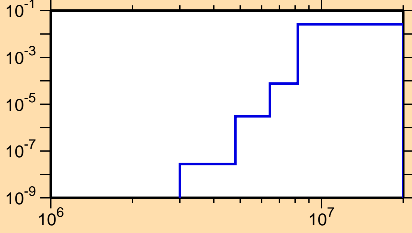
\sigma vs. E for ^{107}\text{Sn}(n,p\alpha)
