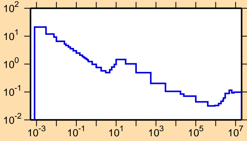
\sigma vs. E for ^{107}\text{Sn}(n,\alpha)
