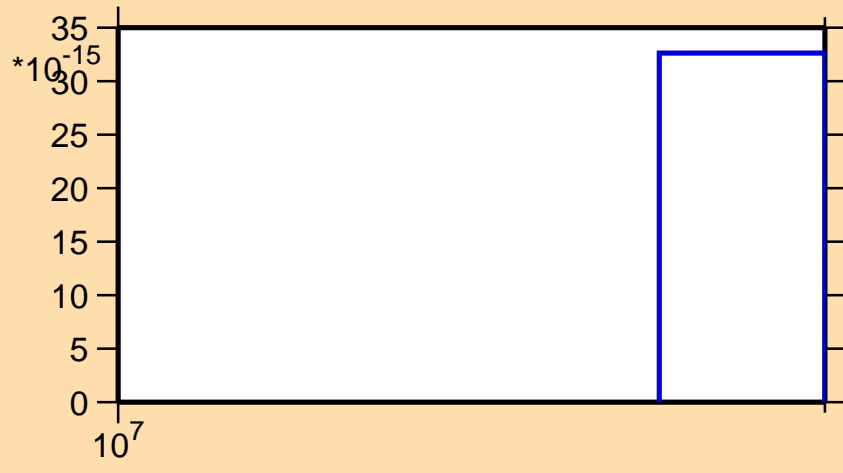
\sigma vs. E for ^{108}\text{Sn}(n,nt)
