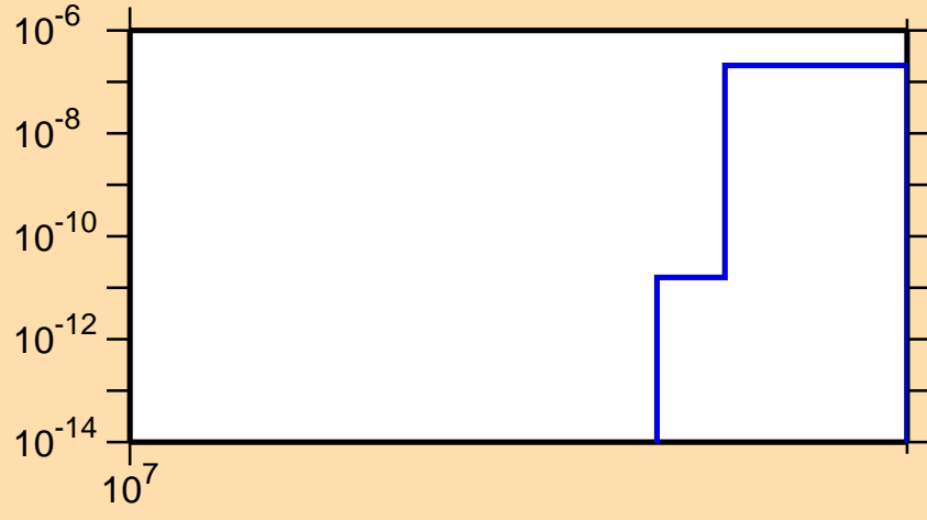
\sigma vs. E for ^{108}\text{Sn}(n,\text{nd})
