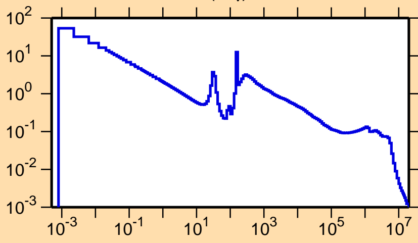
\sigma vs. E for ^{108}\text{Sn}(n,\gamma)
