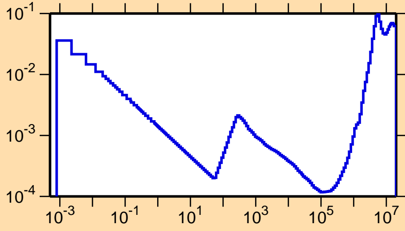
\sigma vs. E for ^{108}\text{Sn}(n,\alpha)
