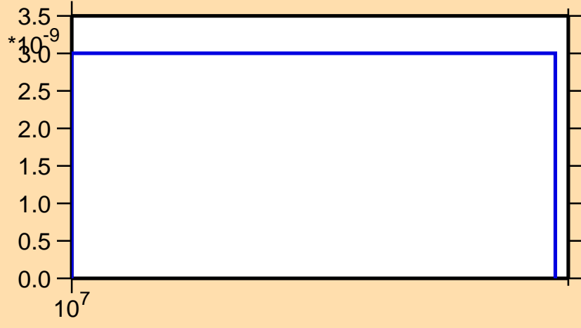
\sigma vs. E for ^{108}\text{Sn} (mt 45)
