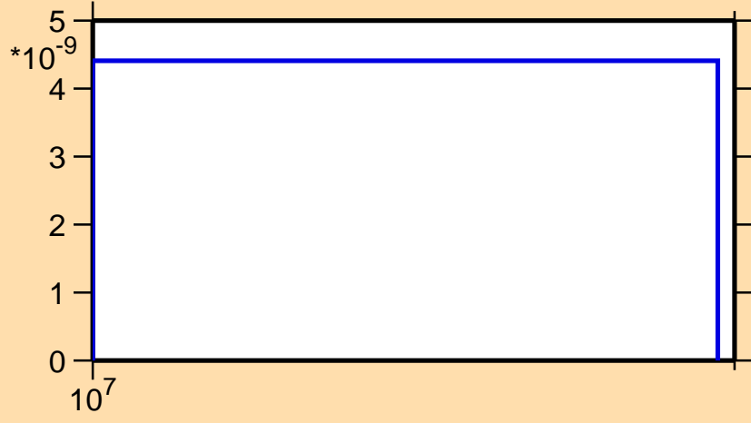
\sigma vs. E for ^{108}\text{Sn}(n,2np)
