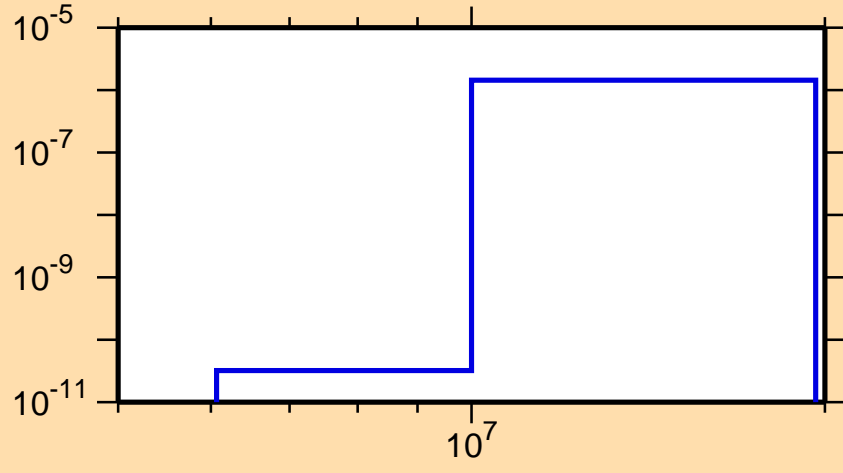
\sigma vs. E for ^{108}\text{Sn}(n,\text{He}3)
