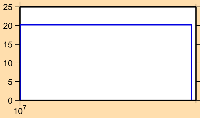
\Delta\sigma/\sigma vs. E for ^{108}\text{Sn}(n,\text{el.})
