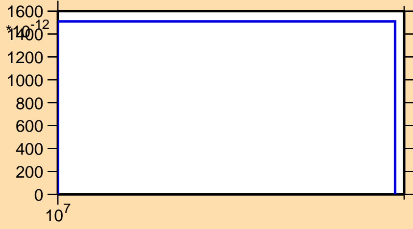
\sigma vs. E for ^{108}\text{Sn}(n,\text{nd})
