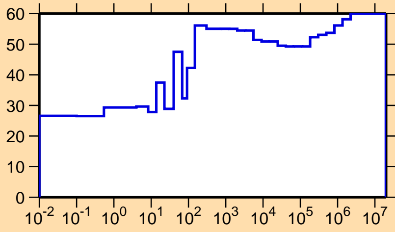
\Delta\sigma/\sigma vs. E for ^{108}\text{Sn}(n,\gamma)
