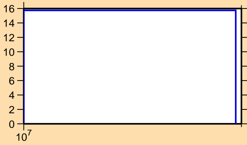
\Delta\sigma/\sigma vs. E for ^{108}\text{Sn}(n,\text{nonel.})
