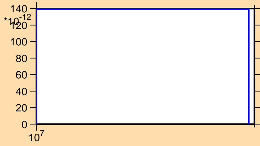
\sigma vs. E for ^{108}\text{Sn}(n,2n\alpha)
