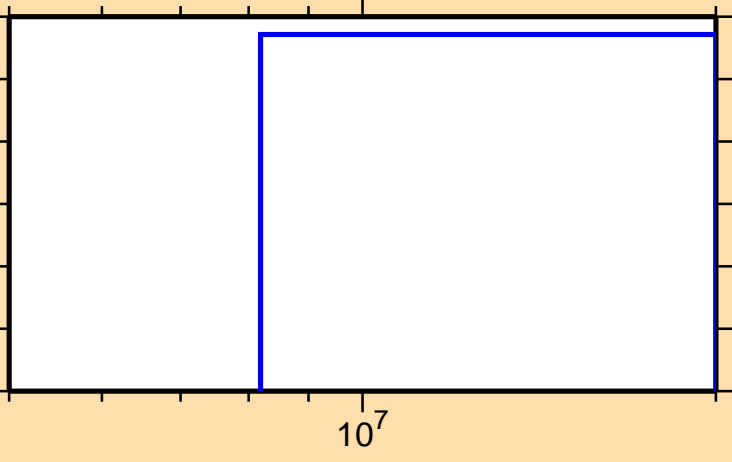
\sigma vs. E for ^{108}\text{Sn}(\text{mt } 45)
