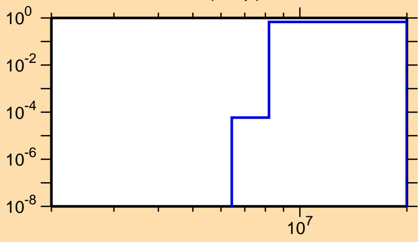
\sigma vs. E for ^{108}\text{Sn}(n,np)
