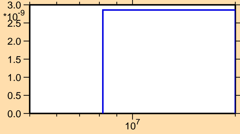
\sigma vs. E for ^{108}\text{Sn}(\text{mt } 45)
