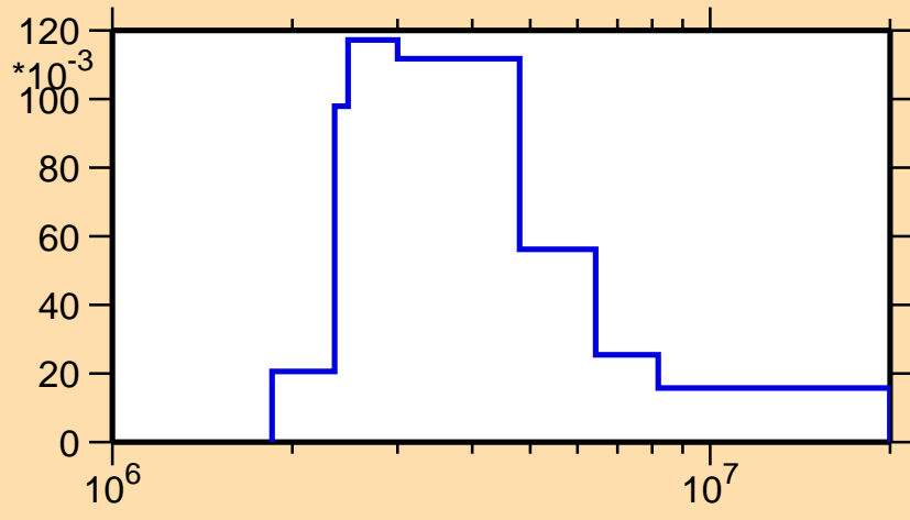
\sigma vs. E for ^{108}\text{Sn}(n,n_2)
