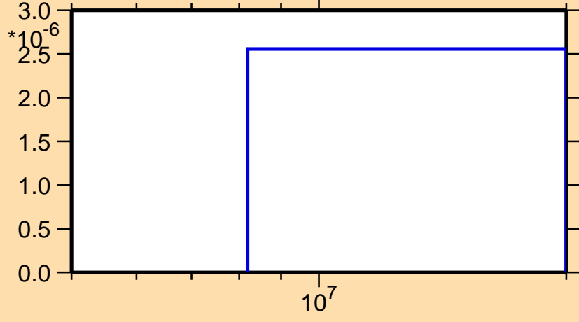
\sigma vs. E for ^{108}\text{Sn}(n,\text{pd})
