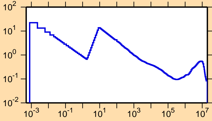
\sigma vs. E for ^{109}\text{Sn}(n,p)
