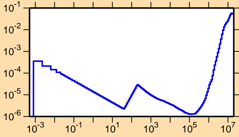
\sigma vs. E for ^{110}\text{Sn}(n,\alpha)
