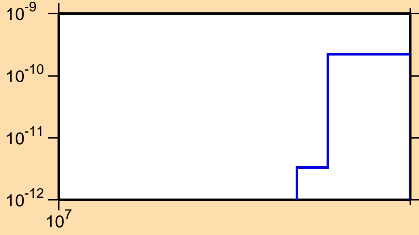
\sigma vs. E for ^{110}\text{Sn}(\text{mt117})
