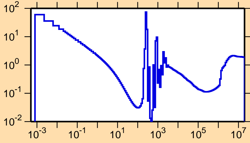
\sigma vs. E for ^{110}\text{Sn}(n,\text{nonel.})
