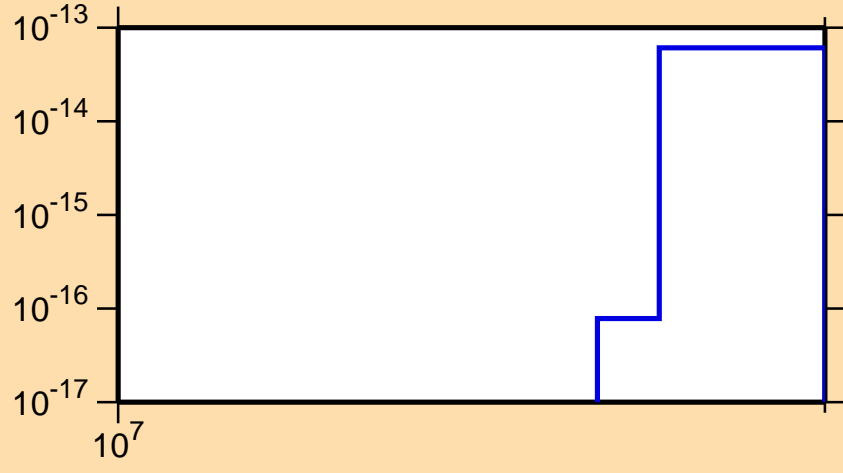
\sigma vs. E for ^{110}\text{Sn} (mt 34)
