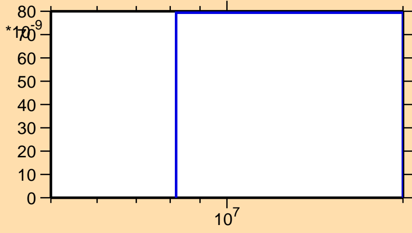
\sigma vs. E for ^{110}\text{Sn}(n,\text{He}3)
