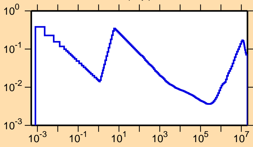
\sigma vs. E for ^{111}\text{Sn}(n,p)
