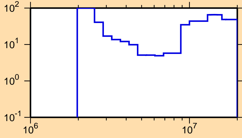
\Delta\sigma/\sigma vs. E for ^{111}\text{Sn}(n,n\text{cont.})
