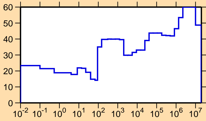
\Delta\sigma/\sigma vs. E for ^{111}\text{Sn}(n,\gamma)
