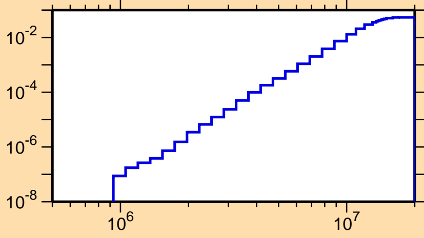
\sigma vs. E for ^{112}\text{Sn}(n,\alpha)
