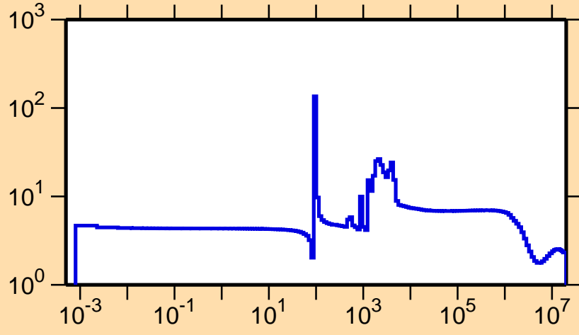
\sigma vs. E for ^{112}\text{Sn}(n,\text{el.})
