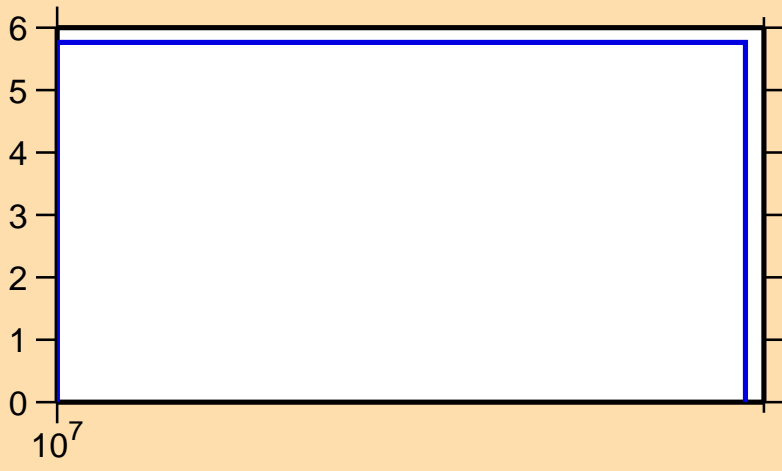
\Delta\sigma/\sigma vs. E for ^{112}\text{Sn}(n,\text{el.})
