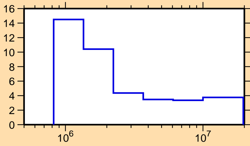
\Delta\sigma/\sigma vs. E for ^{112}\text{Sn}(n,\text{nonel.})
