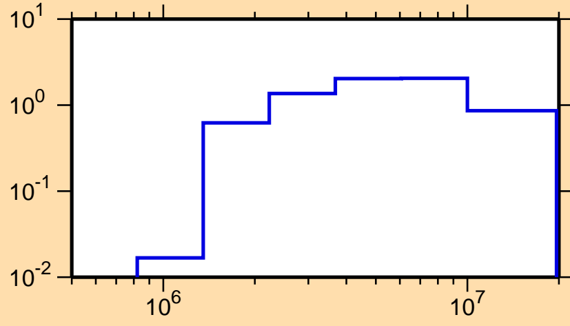
\sigma vs. E for ^{112}\text{Sn}(n,\text{inel.})
