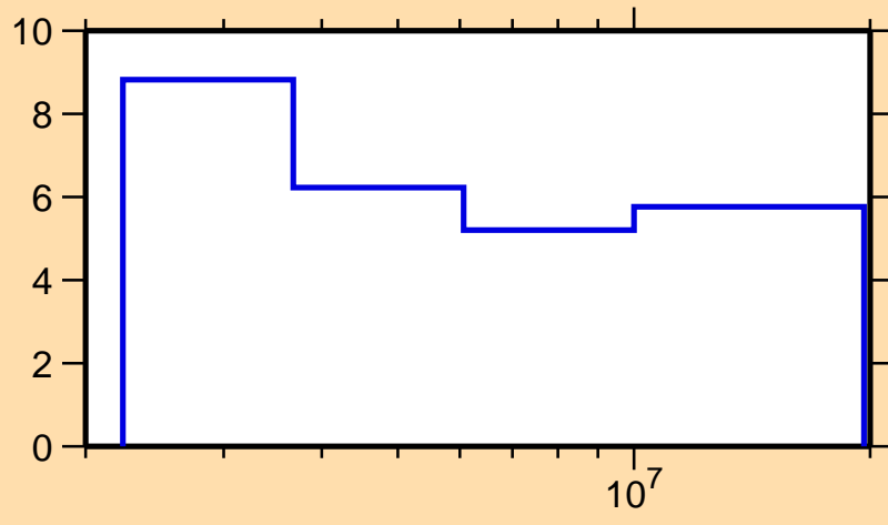
\Delta\sigma/\sigma vs. E for ^{112}\text{Sn}(n,\text{el.})
