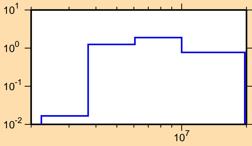
\sigma vs. E for ^{112}\text{Sn}(n,n\text{cont.})
