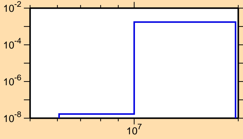
\sigma vs. E for ^{112}\text{Sn}(n,d)
