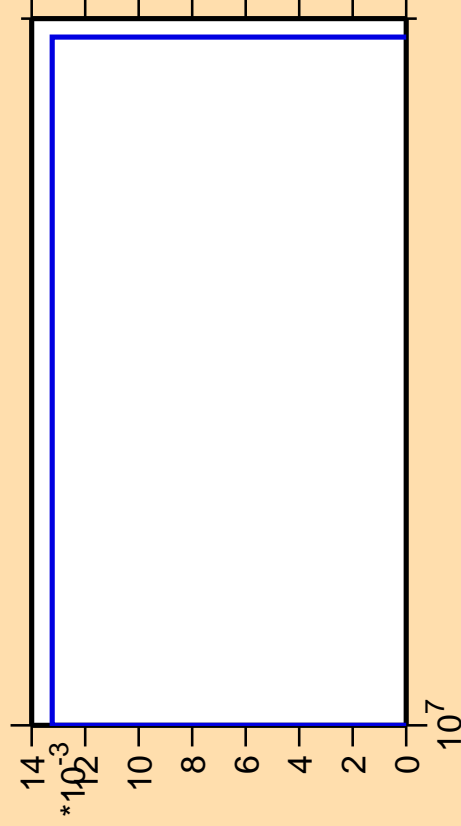
\Delta\sigma/\sigma vs. E for ^{112}\text{Sn} (mt 45)
