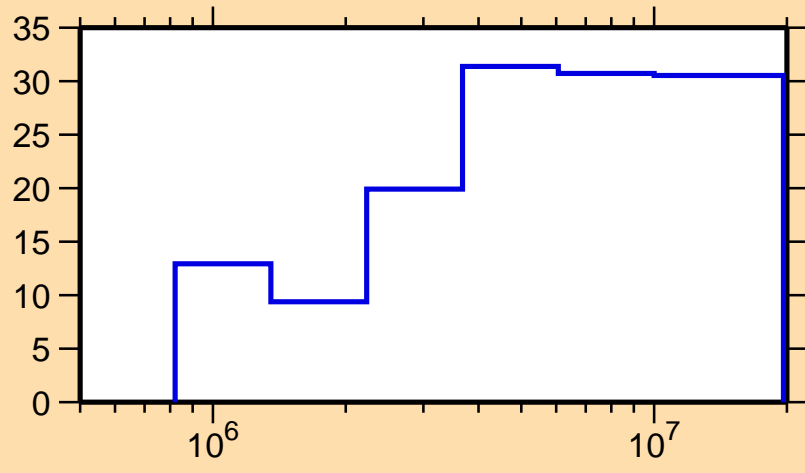
\Delta\sigma/\sigma vs. E for ^{112}\text{Sn}(n,n_1)
