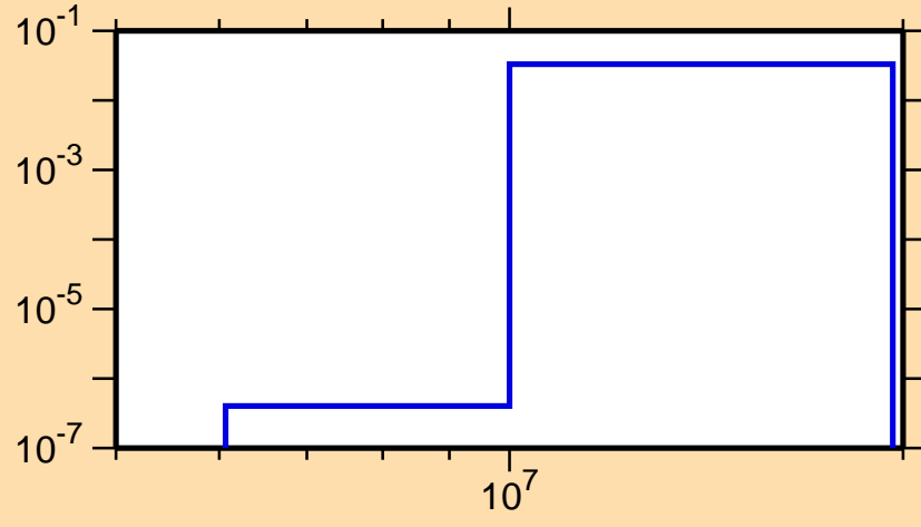
\sigma vs. E for ^{112}\text{Sn}(n,np)
