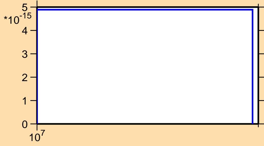
\sigma vs. E for ^{112}\text{Sn} (mt 45)
