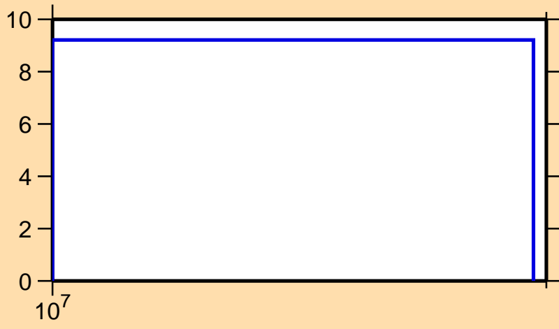
\Delta\sigma/\sigma vs. E for ^{112}\text{Sn}(n,2n)
