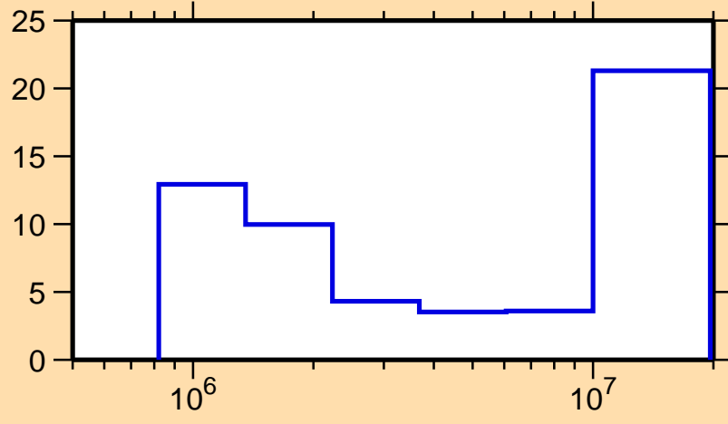
\Delta\sigma/\sigma vs. E for ^{112}\text{Sn}(n,\text{inel.})
