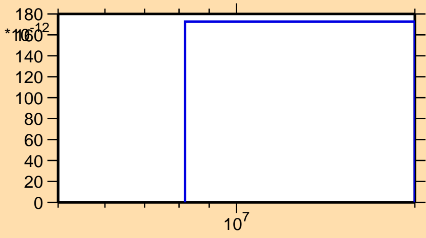
\sigma vs. E for ^{112}\text{Sn}(n,\text{pd})
