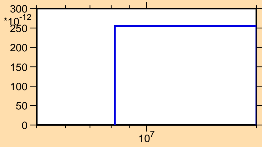
\sigma vs. E for ^{112}\text{Sn}(n,\text{nd})
