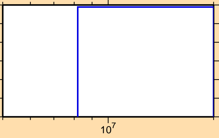
\sigma vs. E for ^{112}\text{Sn}(n,t)
