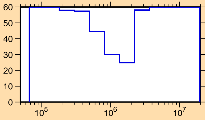
\Delta\sigma/\sigma vs. E for ^{113}\text{Sn}(n,n_1)
