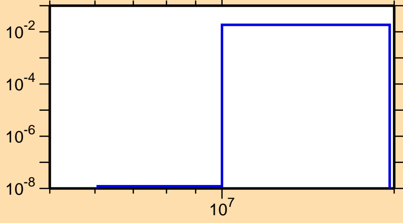
\sigma vs. E for ^{113}\text{Sn}(n,np)
