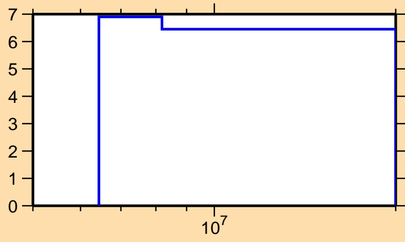
\Delta\sigma/\sigma vs. E for ^{113}\text{Sn}(n,\text{nonel.})
