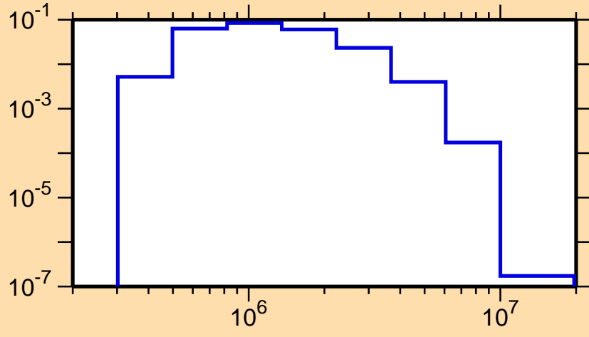
\sigma vs. E for ^{113}\text{Sn}(n,n_3)
