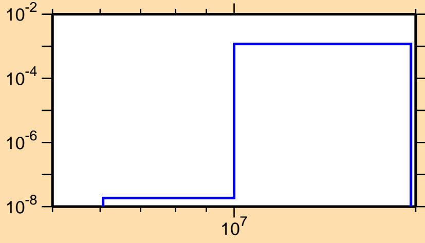
\sigma vs. E for ^{113}\text{Sn}(n,n\alpha)
