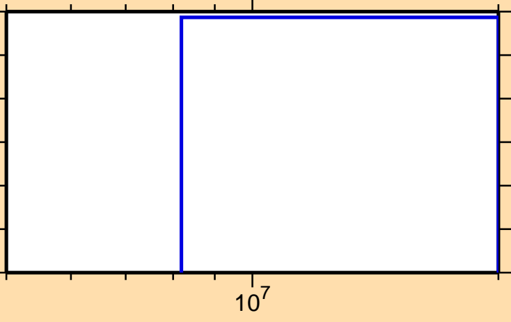
\sigma vs. E for ^{113}\text{Sn}(n,2np)
