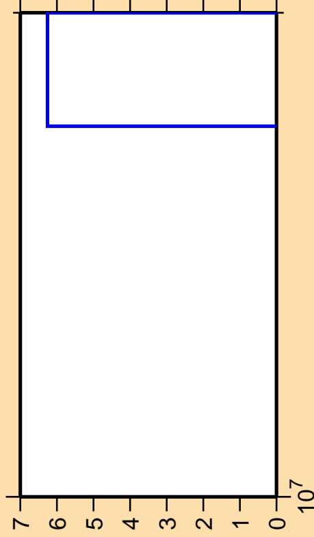
\Delta\sigma/\sigma vs. E for ^{114}\text{Sn}(n,2np)
