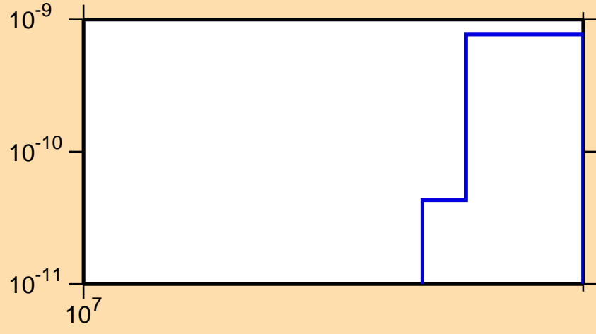
\sigma vs. E for ^{114}\text{Sn}(n,p\alpha)
