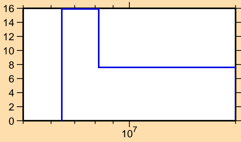
\Delta\sigma/\sigma vs. E for ^{115}\text{Sn}(n,2n)
