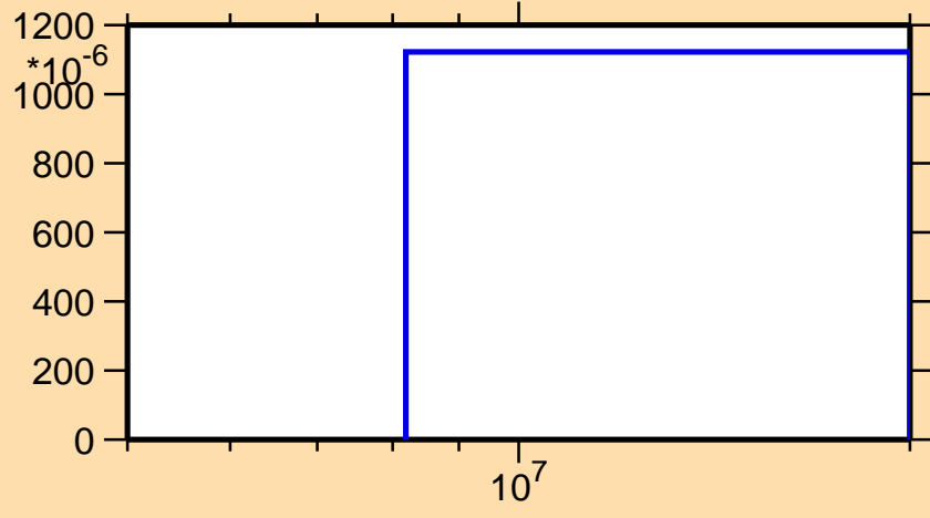
\sigma vs. E for ^{115}\text{Sn}(n,np)
