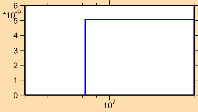
\sigma vs. E for ^{115}\text{Sn}(n,nd)
