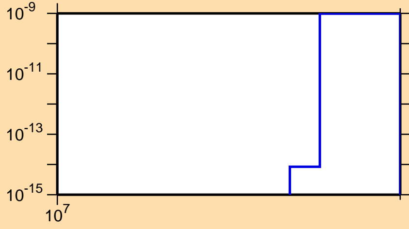
\sigma vs. E for ^{116}\text{Sn}(n,\text{nd})
