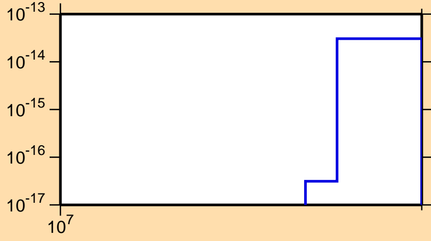
\sigma vs. E for ^{116}\text{Sn}(n,\text{pd})
