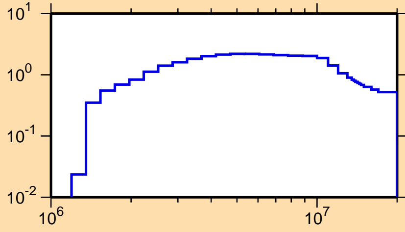
\sigma vs. E for ^{116}\text{Sn}(n,\text{inel.})
