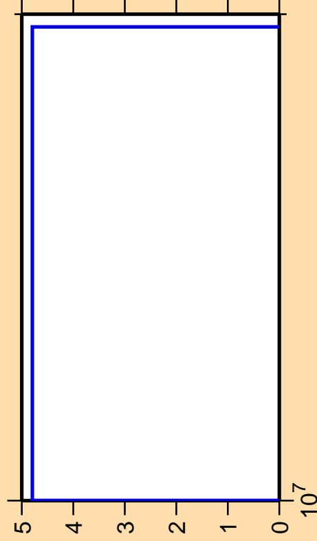
\Delta\sigma/\sigma vs. E for ^{116}\text{Sn}(n,\text{nd})
