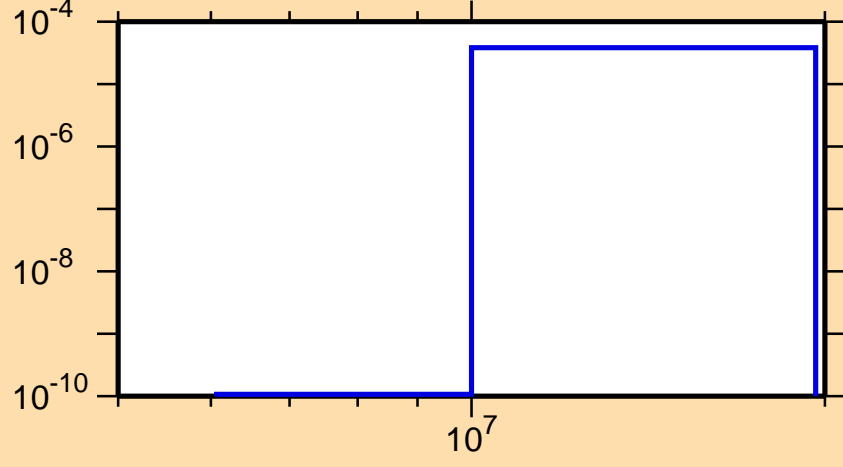
\sigma vs. E for ^{116}\text{Sn}(n,n\alpha)
