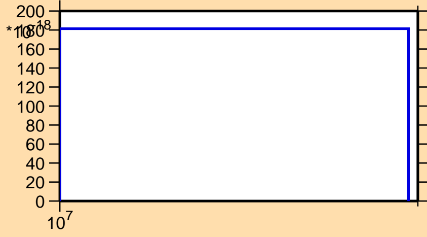
\sigma vs. E for ^{116}\text{Sn}(n,pd)
