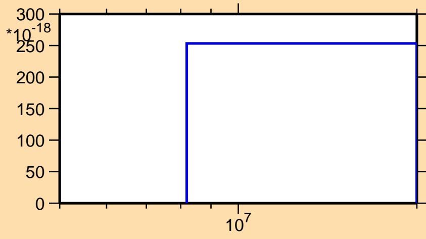
\sigma vs. E for ^{116}\text{Sn}(n,pd)
