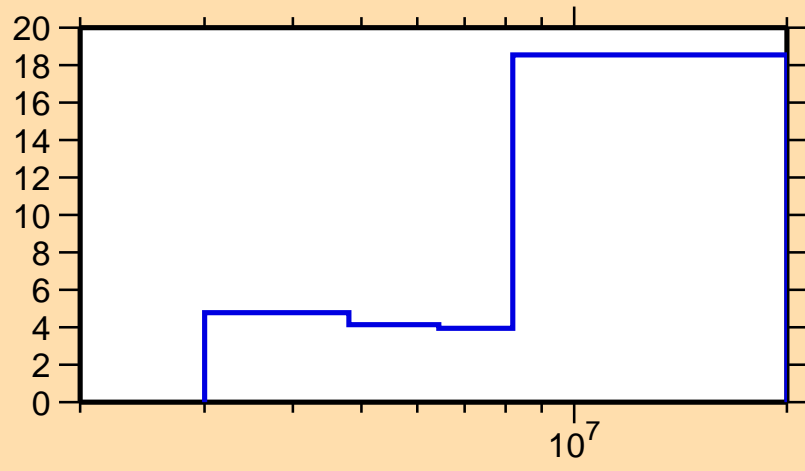
\Delta\sigma/\sigma vs. E for ^{116}\text{Sn}(n,n\text{cont.})
