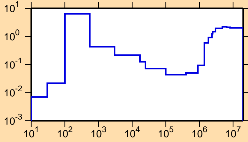
\sigma vs. E for ^{116}\text{Sn}(n,\text{nonel.})
