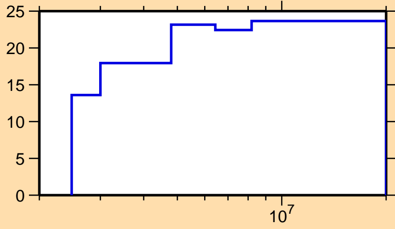
\Delta\sigma/\sigma vs. E for ^{116}\text{Sn}(n,n_1)
