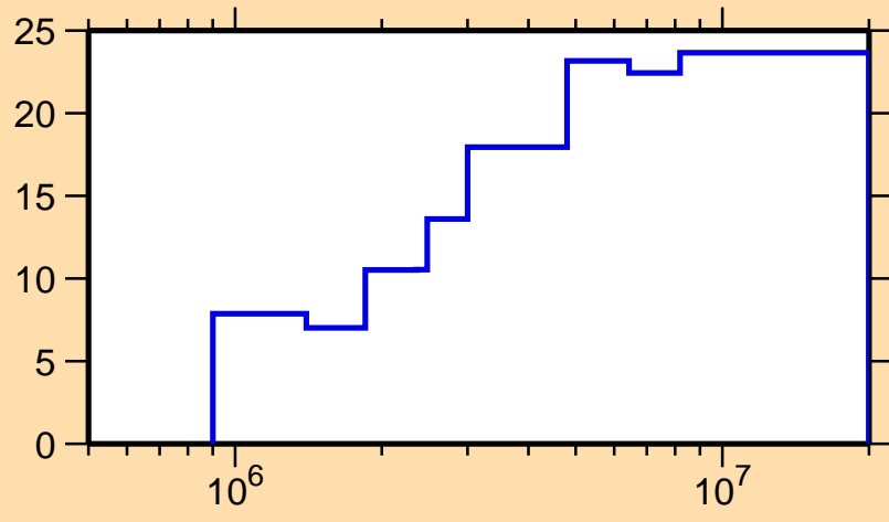
\Delta\sigma/\sigma vs. E for ^{116}\text{Sn}(n,n_1)
