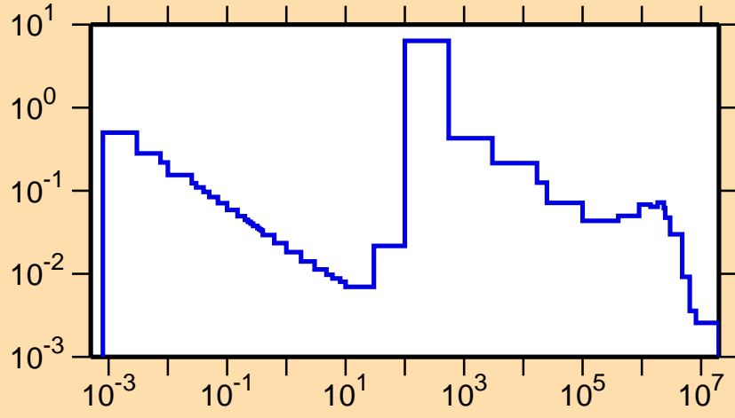
\sigma vs. E for ^{116}\text{Sn}(n,\gamma)
