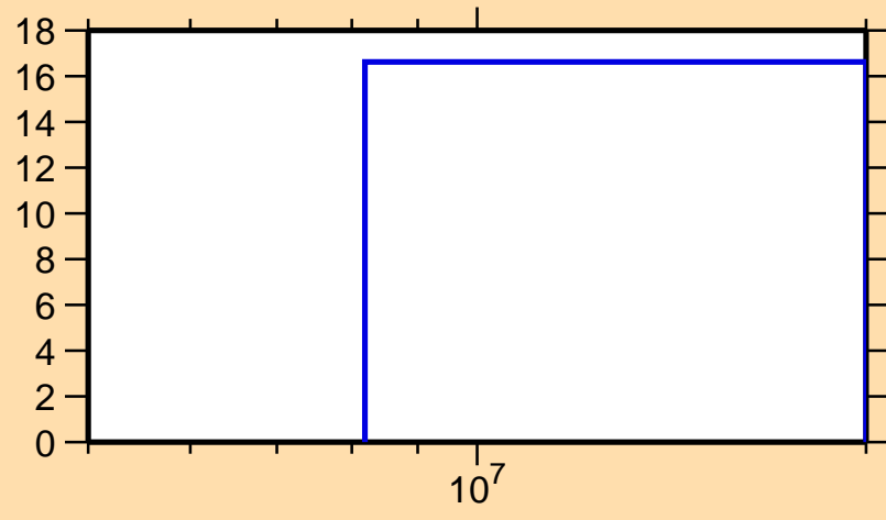
\Delta\sigma/\sigma vs. E for ^{116}\text{Sn}(n,2n)
