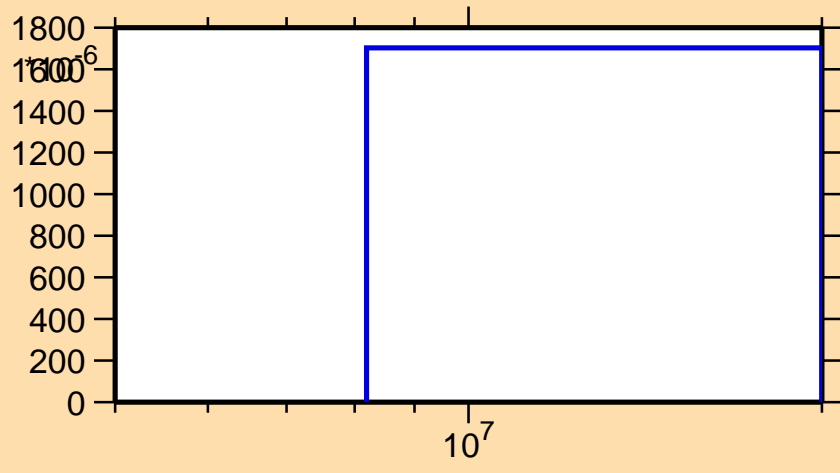
\sigma vs. E for ^{116}\text{Sn}(n,np)
