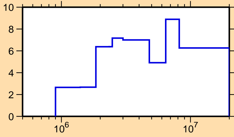
\Delta\sigma/\sigma vs. E for ^{116}\text{Sn}(n,\text{el.})
