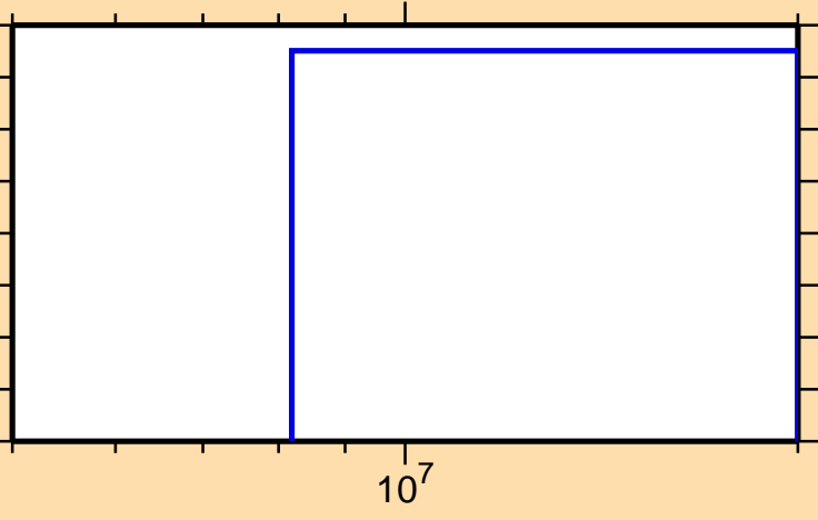
\sigma vs. E for ^{116}\text{Sn}(n,3n)
