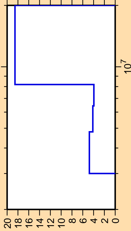
\Delta\sigma/\sigma vs. E for ^{116}\text{Sn}(n,n\text{cont.})
