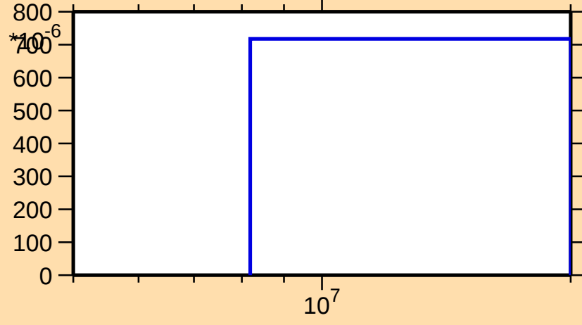
\sigma vs. E for ^{117}\text{Sn}(n,np)
