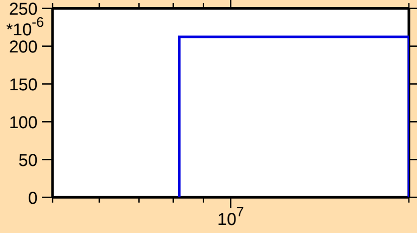
\sigma vs. E for ^{117}\text{Sn}(n,3n)
