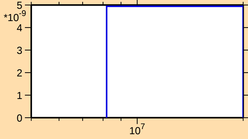
\sigma vs. E for ^{117}\text{Sn}(n,\text{nd})
