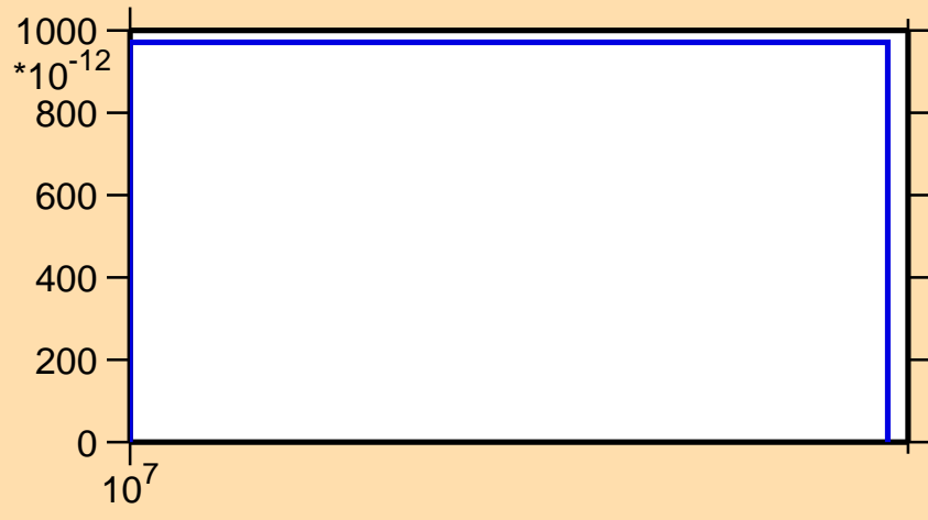
\sigma vs. E for ^{117}\text{Sn}(n,2np)
