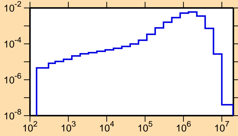
\sigma vs. E for ^{117}\text{Sn}(n,n_1)
