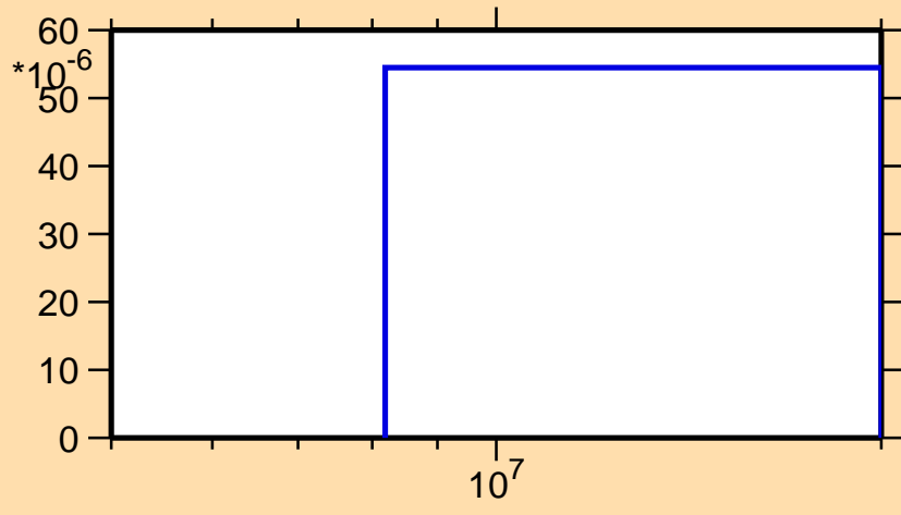
\sigma vs. E for ^{117}\text{Sn}(n,n\alpha)
