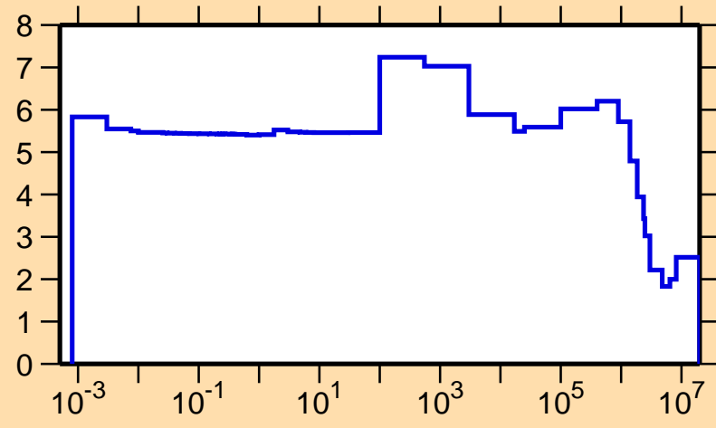
\sigma vs. E for ^{117}\text{Sn}(n,\text{el.})
