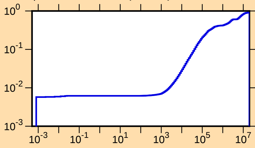
\mu vs. E for ^{118}\text{Sn}(\text{mt251})
