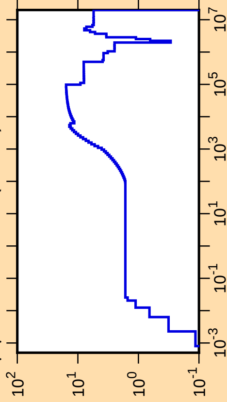
\Delta\mu/\mu vs. E for ^{118}\text{Sn}(\text{mt251})
