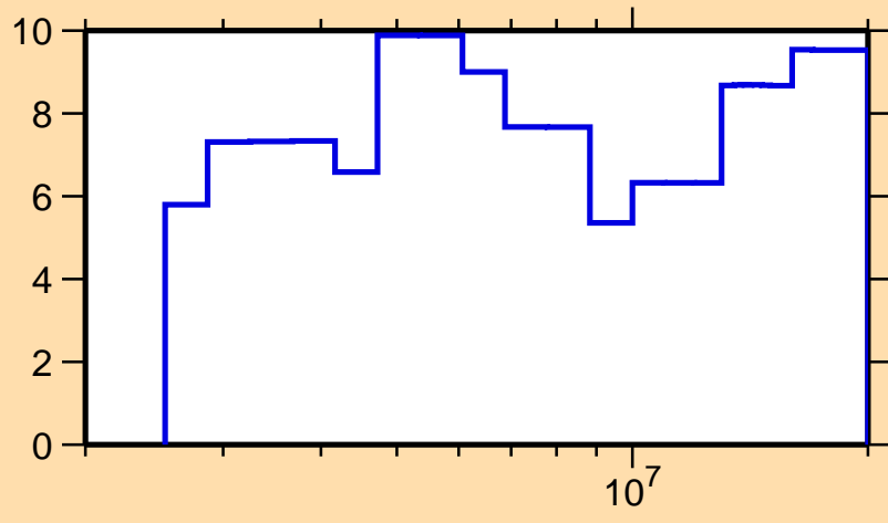
\Delta\sigma/\sigma vs. E for ^{119}\text{Sn}(n,el.)
