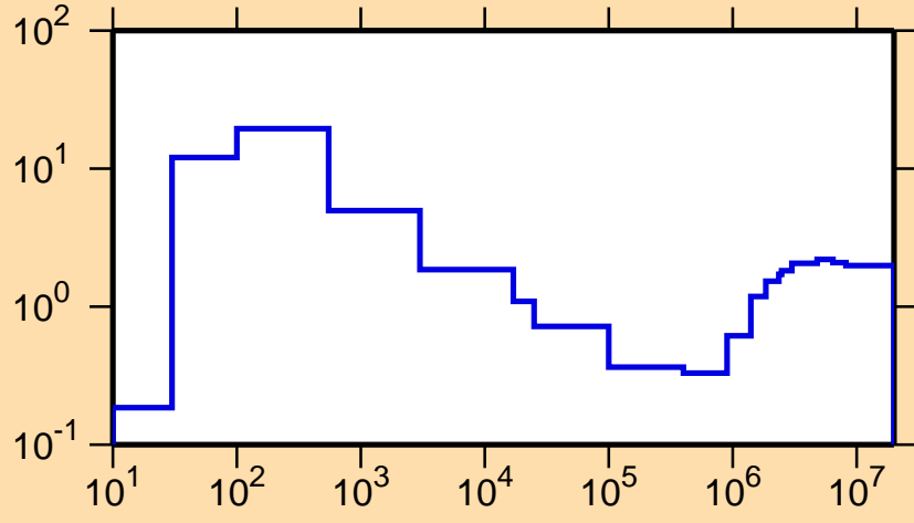
\sigma vs. E for ^{119}\text{Sn}(n,\text{nonel.})
