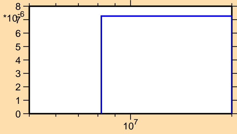
\sigma vs. E for ^{119}\text{Sn}(n,t)
