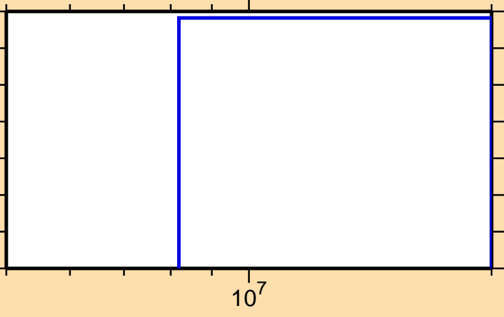
\sigma vs. E for ^{119}\text{Sn}(n,\text{He}3)
