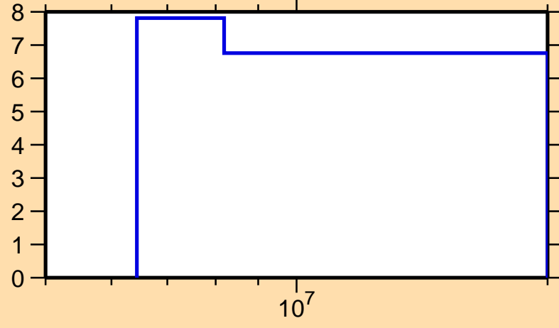
\Delta\sigma/\sigma vs. E for ^{119}\text{Sn}(n,\text{el.})
