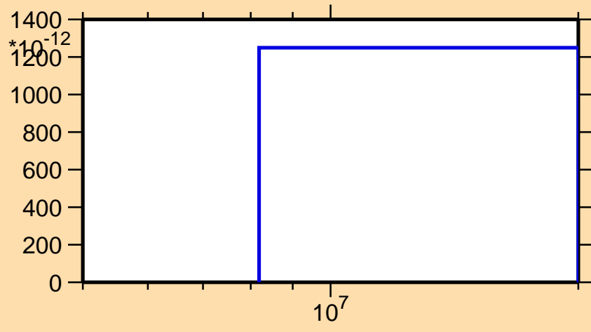
\sigma vs. E for ^{119}\text{Sn}(n,\text{nd})
