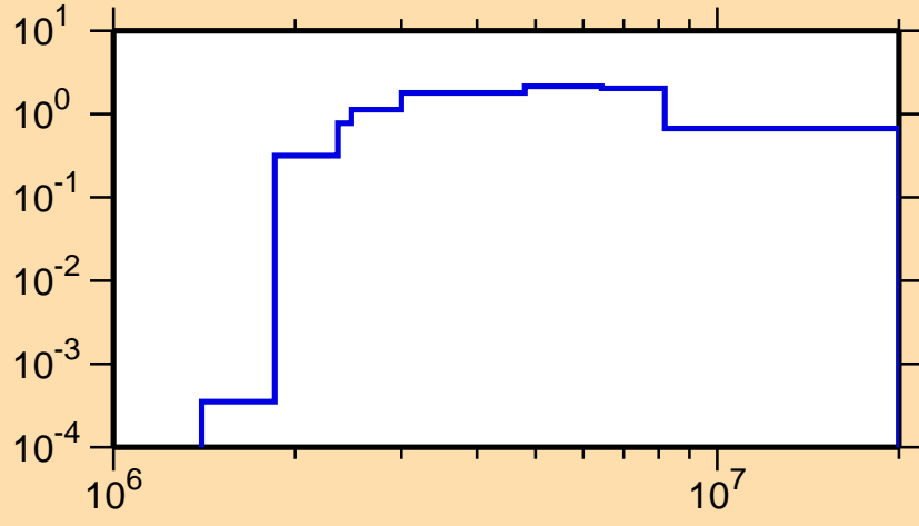
\sigma vs. E for ^{119}\text{Sn}(n,n\text{cont.})
