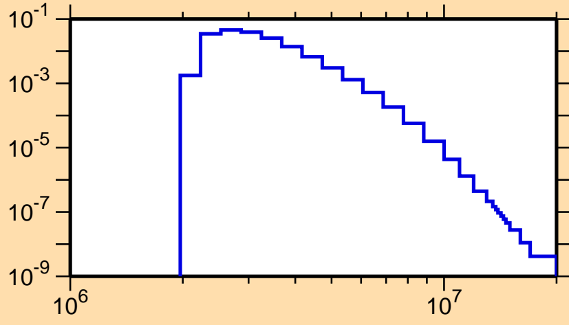
\sigma vs. E for ^{120}\text{Sn}(n,n_4)
