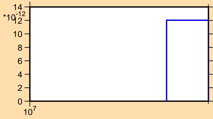
\sigma vs. E for ^{120}\text{Sn}(n,\text{nd})
