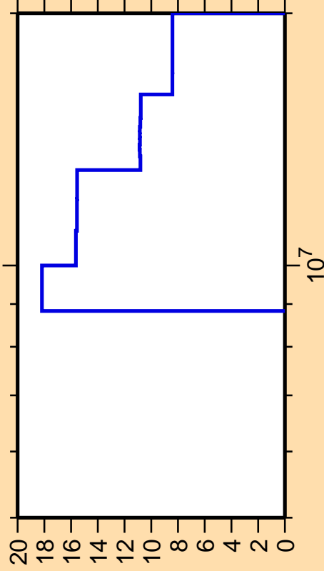
\Delta\sigma/\sigma vs. E for ^{120}\text{Sn}(n,2n)
