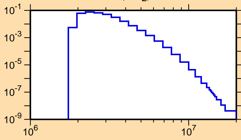
\sigma vs. E for ^{120}\text{Sn}(n,n_2)
