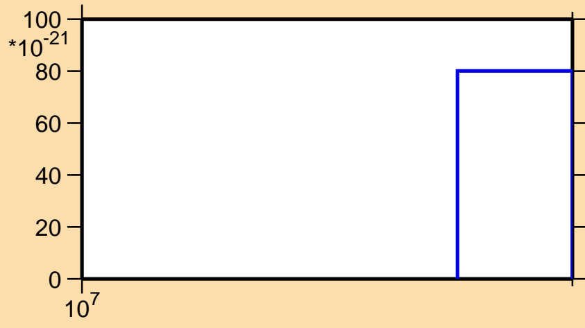
\sigma vs. E for ^{120}\text{Sn}(n,2np)
