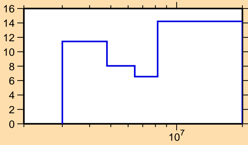
\Delta\sigma/\sigma vs. E for ^{120}\text{Sn}(n,n\text{cont.})
