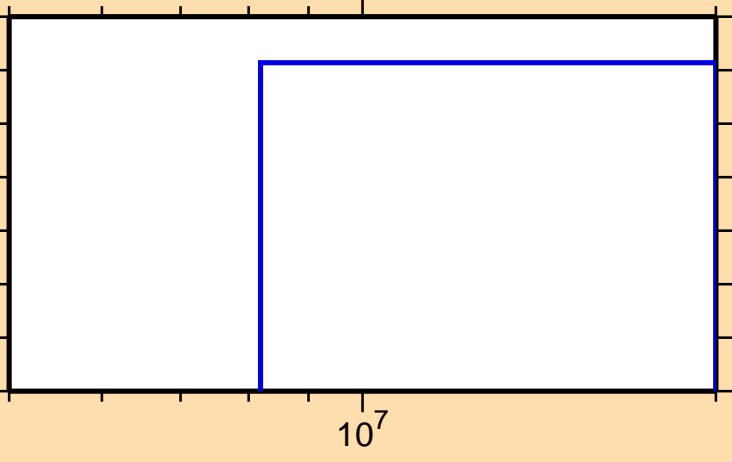
\sigma vs. E for ^{120}\text{Sn}(n,n\alpha)
