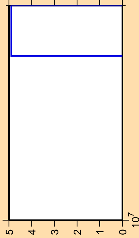
\Delta\sigma/\sigma vs. E for ^{121}\text{Sn}(n,nt)
