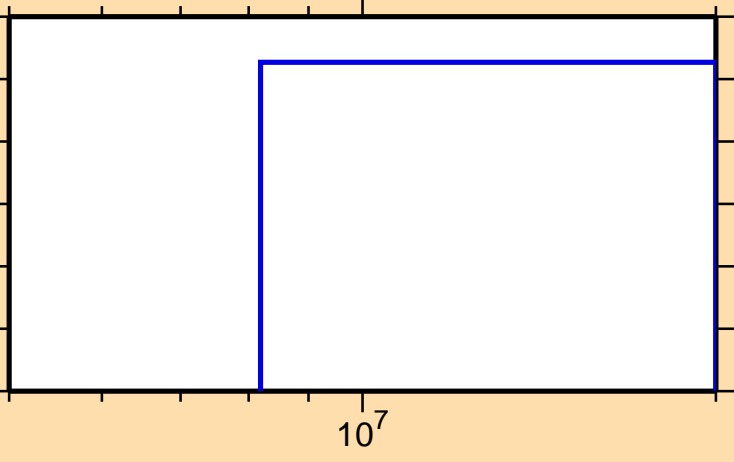
\sigma vs. E for ^{121}\text{Sn}(n,n\alpha)
