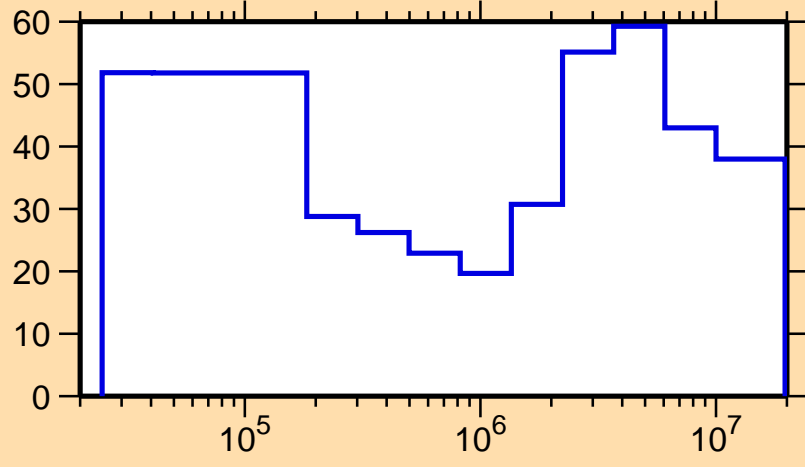
\Delta\sigma/\sigma vs. E for ^{123}\text{Sn}(n,n_1)
