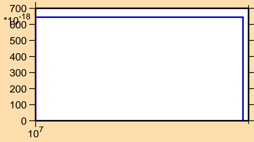
\sigma vs. E for ^{123}\text{Sn}(n,nt)
