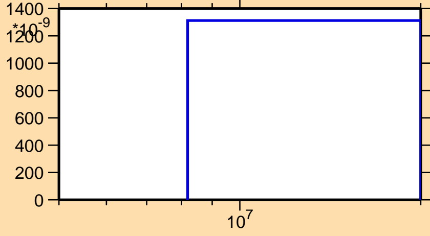
\sigma vs. E for ^{123}\text{Sn}(n,t)
