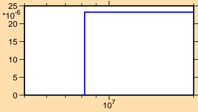
\sigma vs. E for ^{123}\text{Sn}(n,d)
