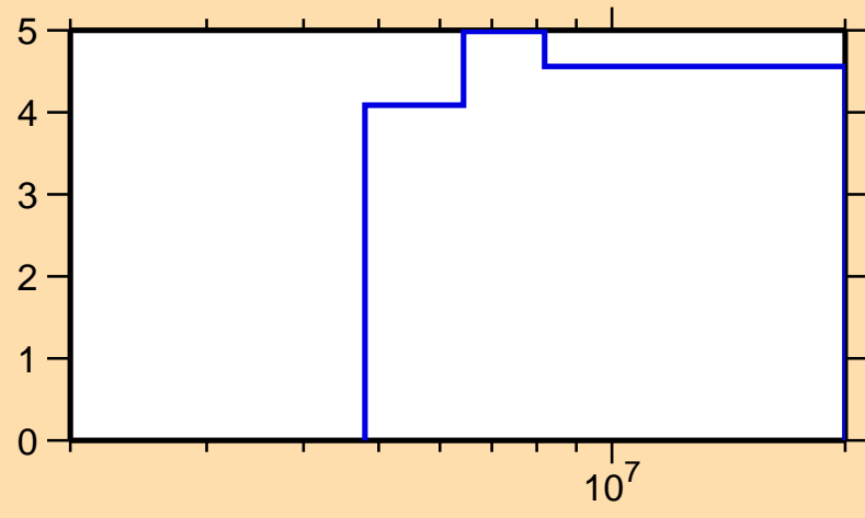
\Delta\sigma/\sigma vs. E for ^{123}\text{Sn}(n,\text{tot.})
