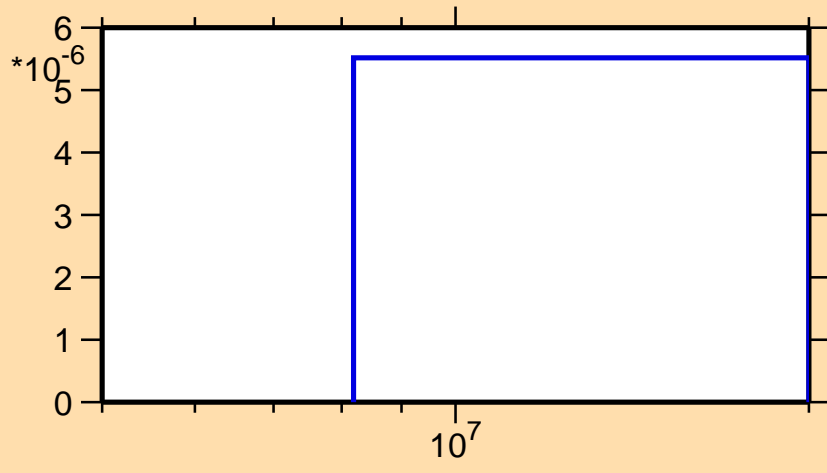
\sigma vs. E for ^{123}\text{Sn}(n,np)
