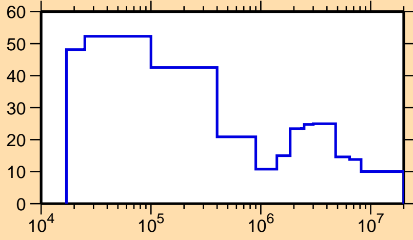
\Delta\sigma/\sigma vs. E for ^{123}\text{Sn}(n,\text{el.})
