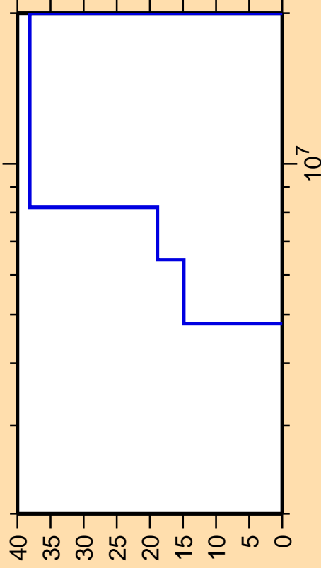
\Delta\sigma/\sigma vs. E for ^{123}\text{Sn}(n,n\text{cont.})
