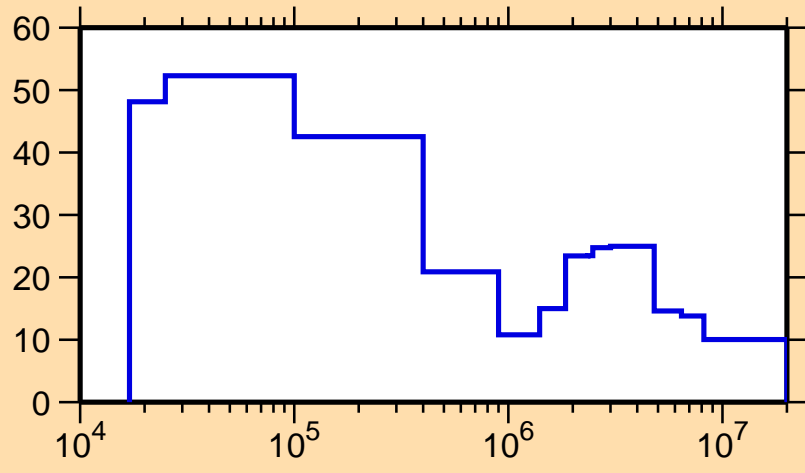
\Delta\sigma/\sigma vs. E for ^{123}\text{Sn}(n,\text{el.})
