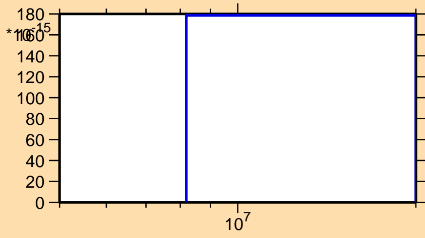
\sigma vs. E for ^{123}\text{Sn}(n,2np)
