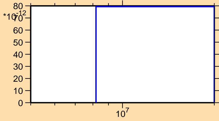
\sigma vs. E for ^{123}\text{Sn}(n,nd)
