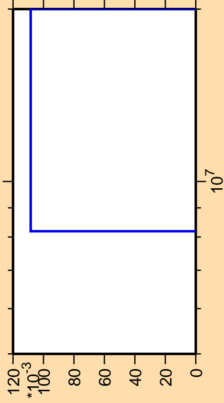
\Delta\sigma/\sigma vs. E for ^{123}\text{Sn}(n,2n\alpha)
