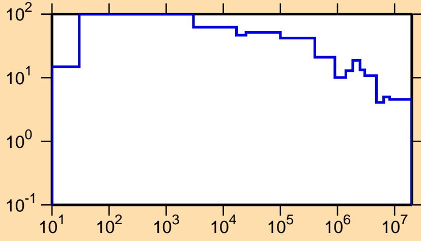
\Delta\sigma/\sigma vs. E for ^{123}\text{Sn}(n,\text{tot.})
