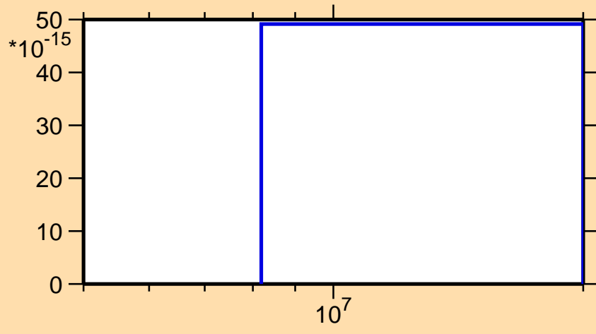
\sigma vs. E for ^{123}\text{Sn}(n,2n\alpha)
