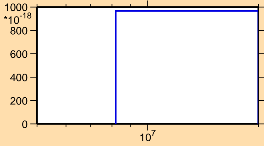
\sigma vs. E for ^{123}\text{Sn}(n,nt)
