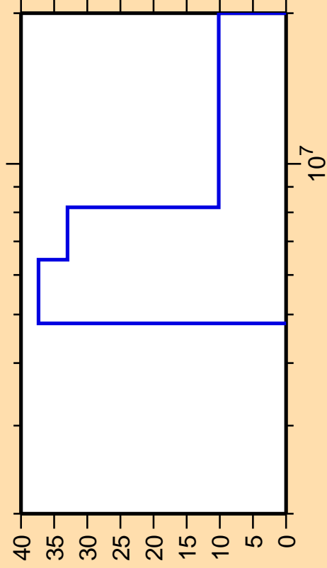
\Delta\sigma/\sigma vs. E for ^{123}\text{Sn}(n,2n)
