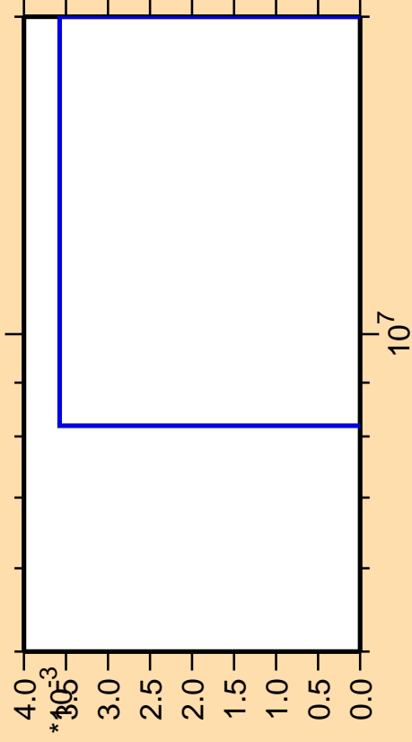
\Delta\sigma/\sigma vs. E for ^{123}\text{Sn}(n,nt)
