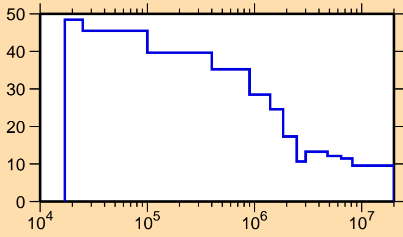
\Delta\sigma/\sigma vs. E for ^{123}\text{Sn}(n,\text{nonel.})
