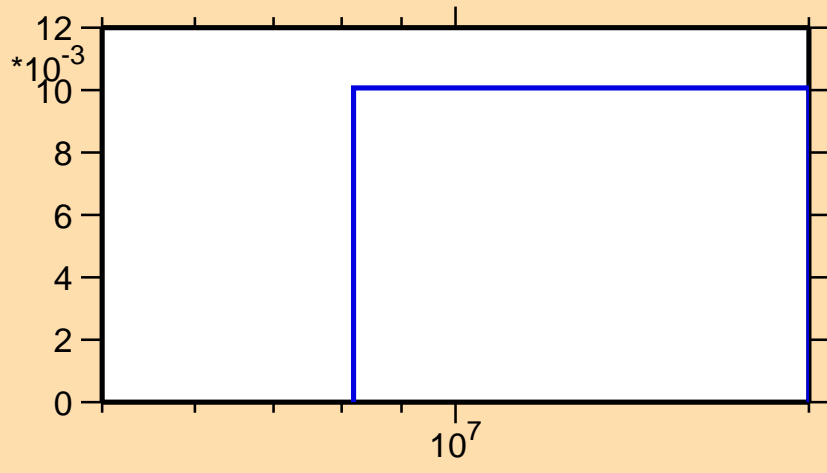
\sigma vs. E for ^{123}\text{Sn}(n,3n)
