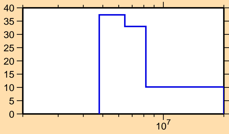
\Delta\sigma/\sigma vs. E for ^{123}\text{Sn}(n,2n)
