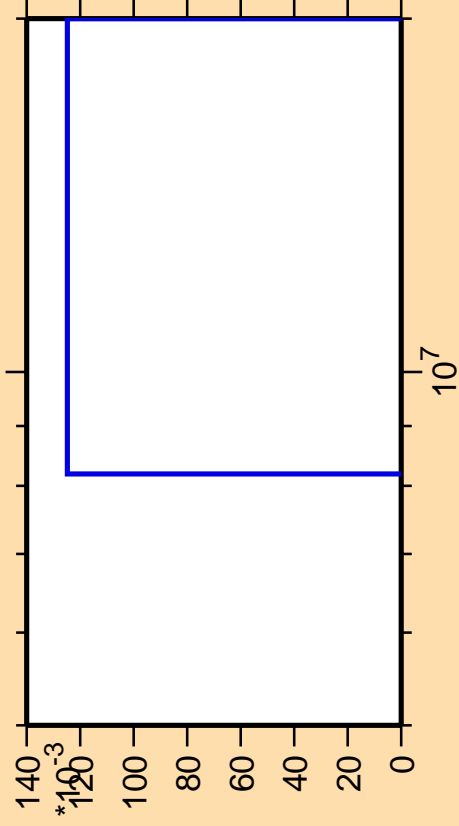
\Delta\sigma/\sigma vs. E for ^{123}\text{Sn}(n,2np)
