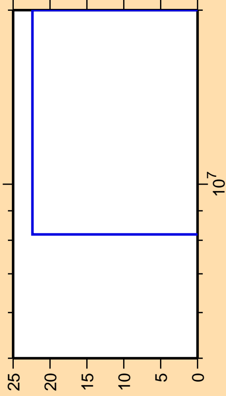
\Delta\sigma/\sigma vs. E for ^{123}\text{Sn}(n,3n)
