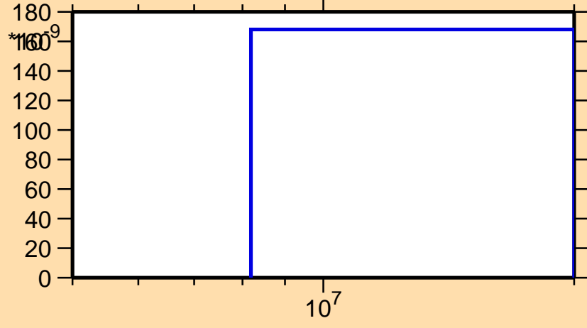
\sigma vs. E for ^{123}\text{Sn}(n,n\alpha)
