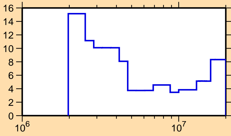
\Delta\sigma/\sigma vs. E for ^{123}\text{Sn}(n,\text{tot.})
