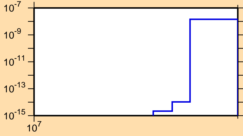
\sigma vs. E for ^{123}\text{Sn}(n,nd)
