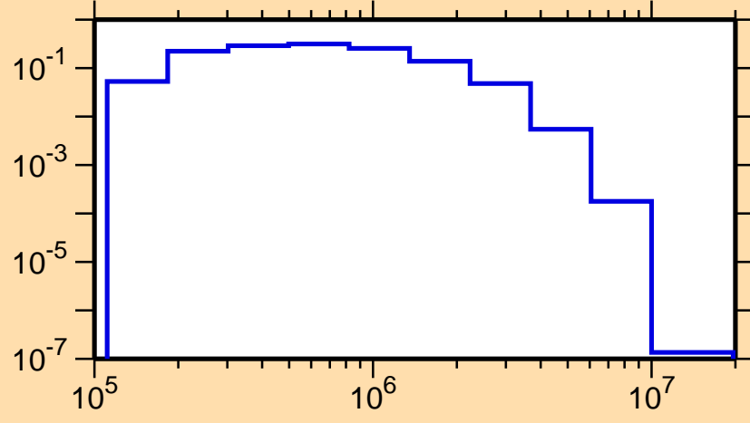
\sigma vs. E for ^{123}\text{Sn}(n,n_2)
