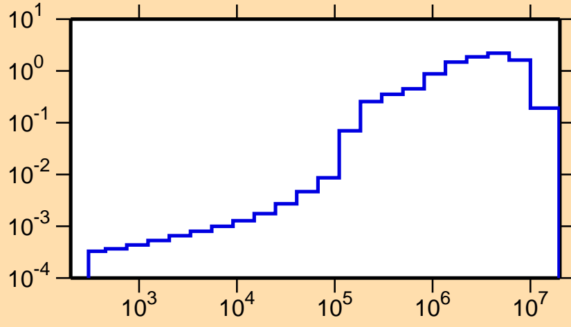
\sigma vs. E for ^{123}\text{Sn}(n,\text{inel.})
