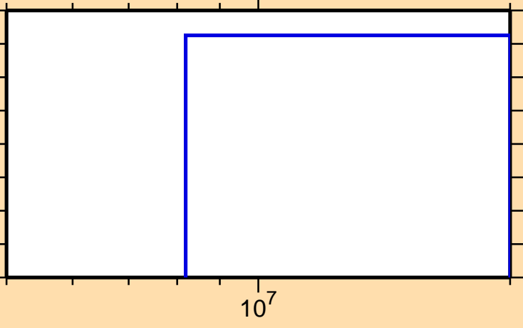
\sigma vs. E for ^{123}\text{Sn}(n,np)
