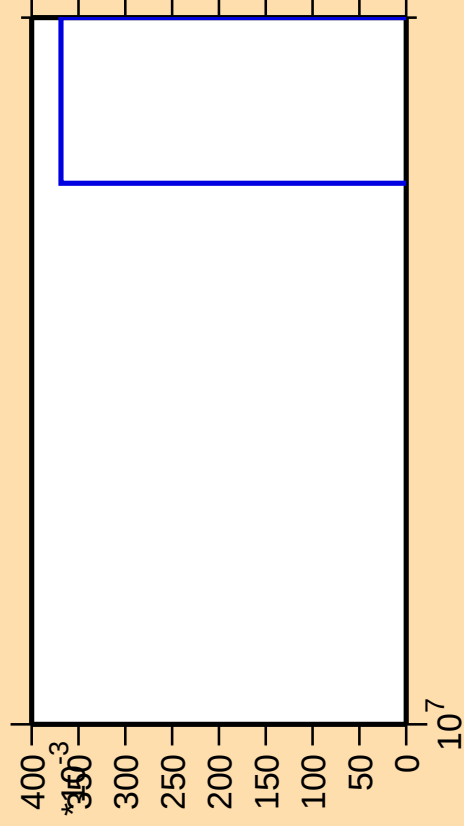
\Delta\sigma/\sigma vs. E for ^{125}\text{Sn}(n,\text{nt})
