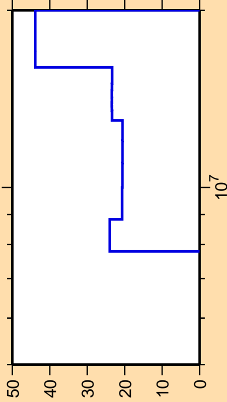
\Delta\sigma/\sigma vs. E for ^{128}\text{Sn}(n,2n)
