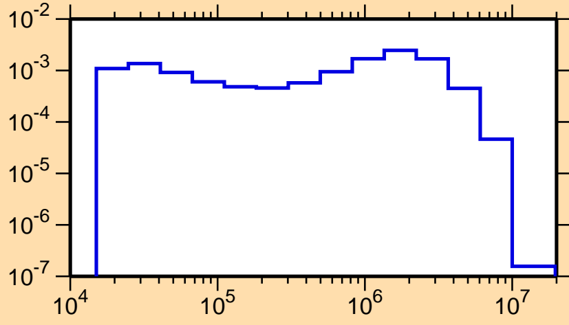
\sigma vs. E for ^{128}\text{Sn}(n,n_1)
