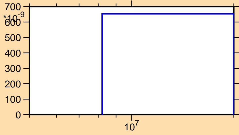
\sigma vs. E for ^{128}\text{Sn}(n,\alpha)
