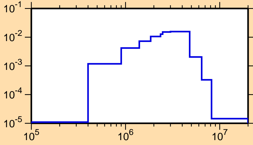
\sigma vs. E for ^{129}\text{Sn}(n,n_2)
