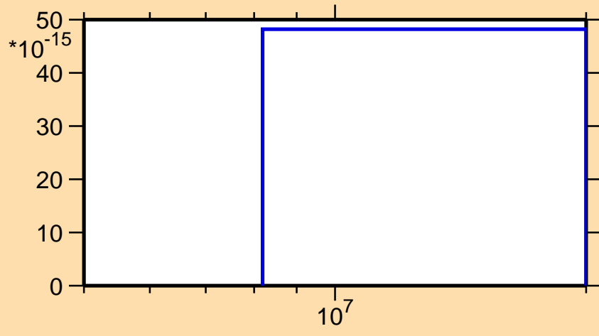
\sigma vs. E for ^{129}\text{Sn}(n,nd)
