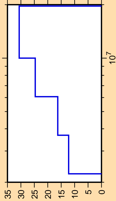
\Delta\sigma/\sigma vs. E for ^{130}\text{Sn}(n,n_4)
