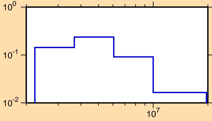
\sigma vs. E for ^{130}\text{Sn}(n,n_3)
