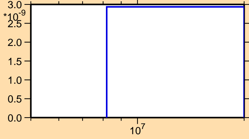
\sigma vs. E for ^{130}\text{Sn}(n,\alpha)
